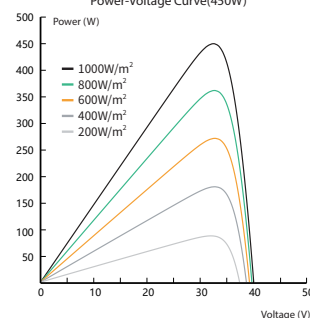
Power-Voltage Curve(450W)
