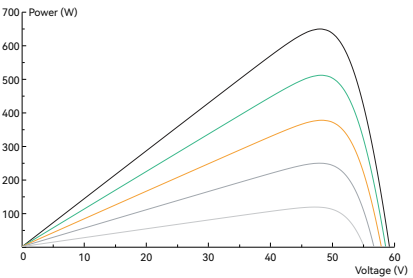
Power-Voltage Curve (650W)
