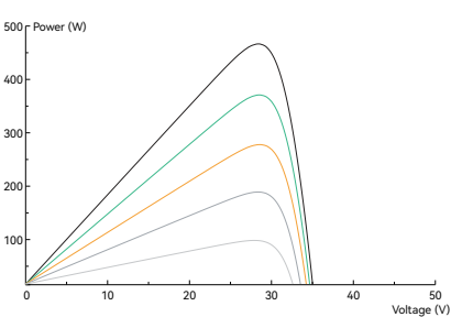
Power-Voltage Curve (460W)
