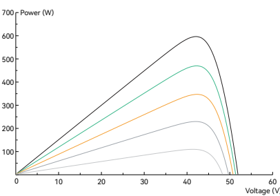
Power-Voltage Curve (595W)
